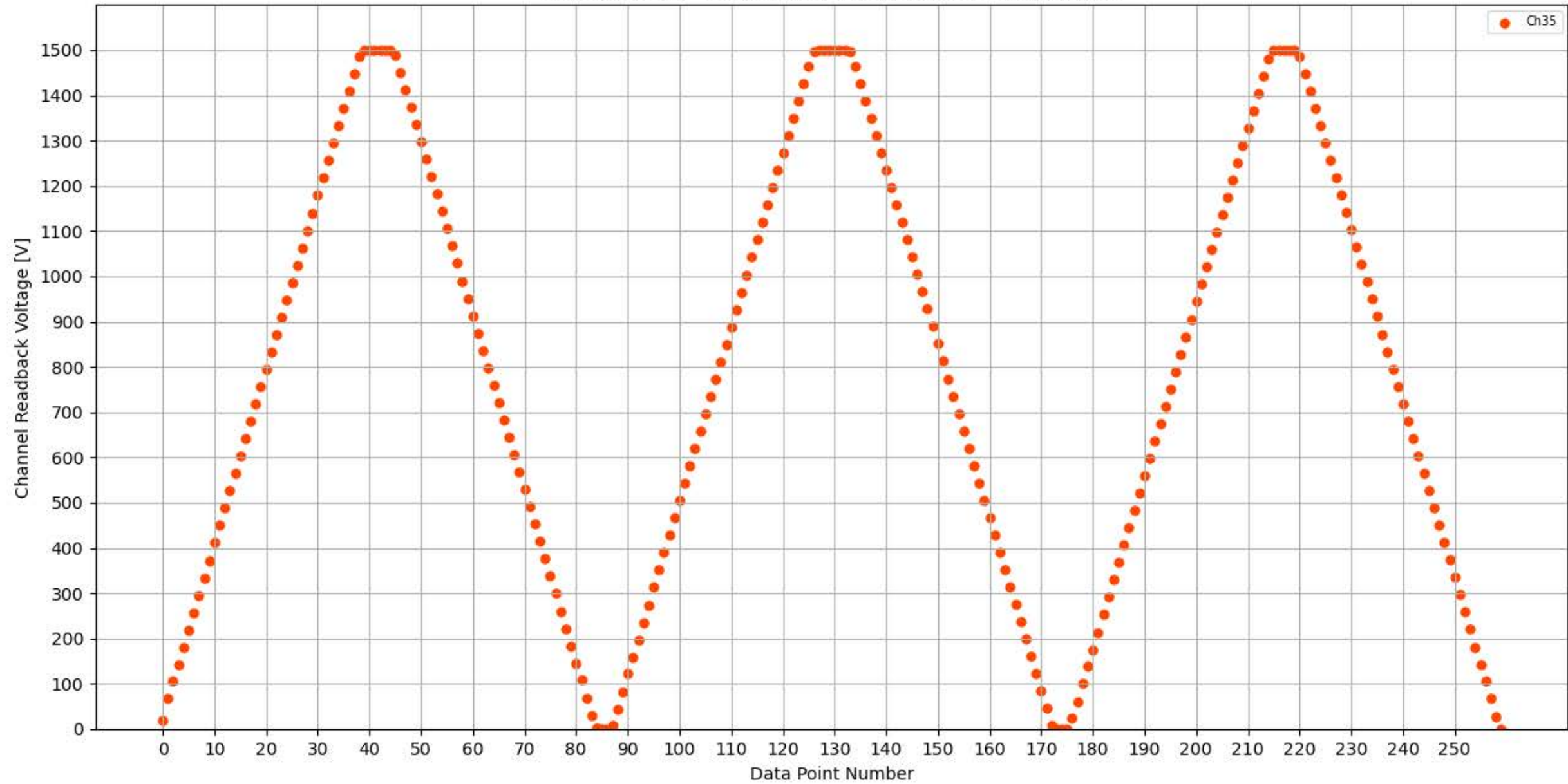
Voltage Ramp Test (Python) Bd #336, Slot #15, Ch #35
