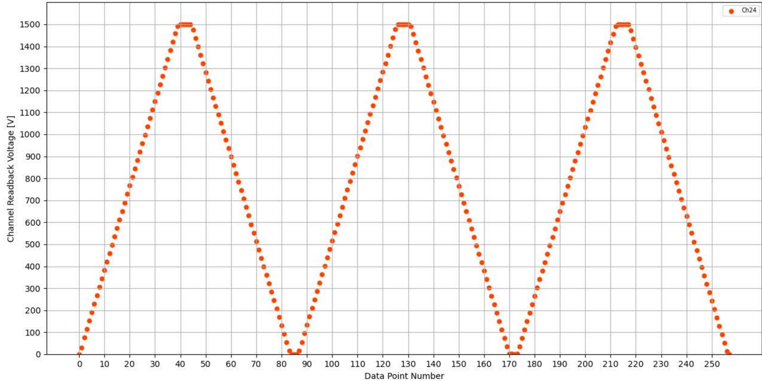
Voltage Ramp Test (Python) Bd #336, Slot #15, Ch #24
