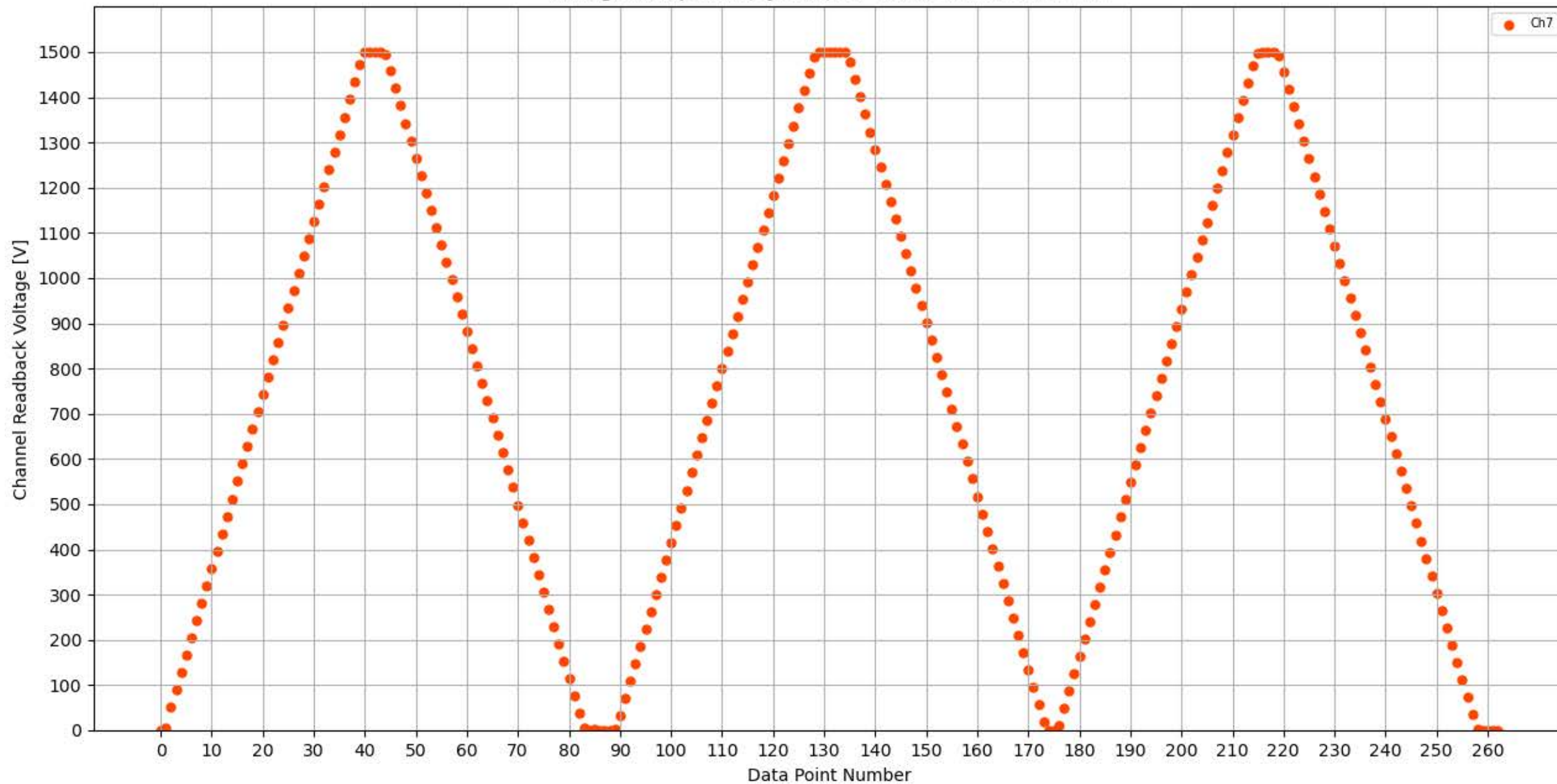
Voltage Ramp Test (Python) Bd #336, Slot #15, Ch #7
