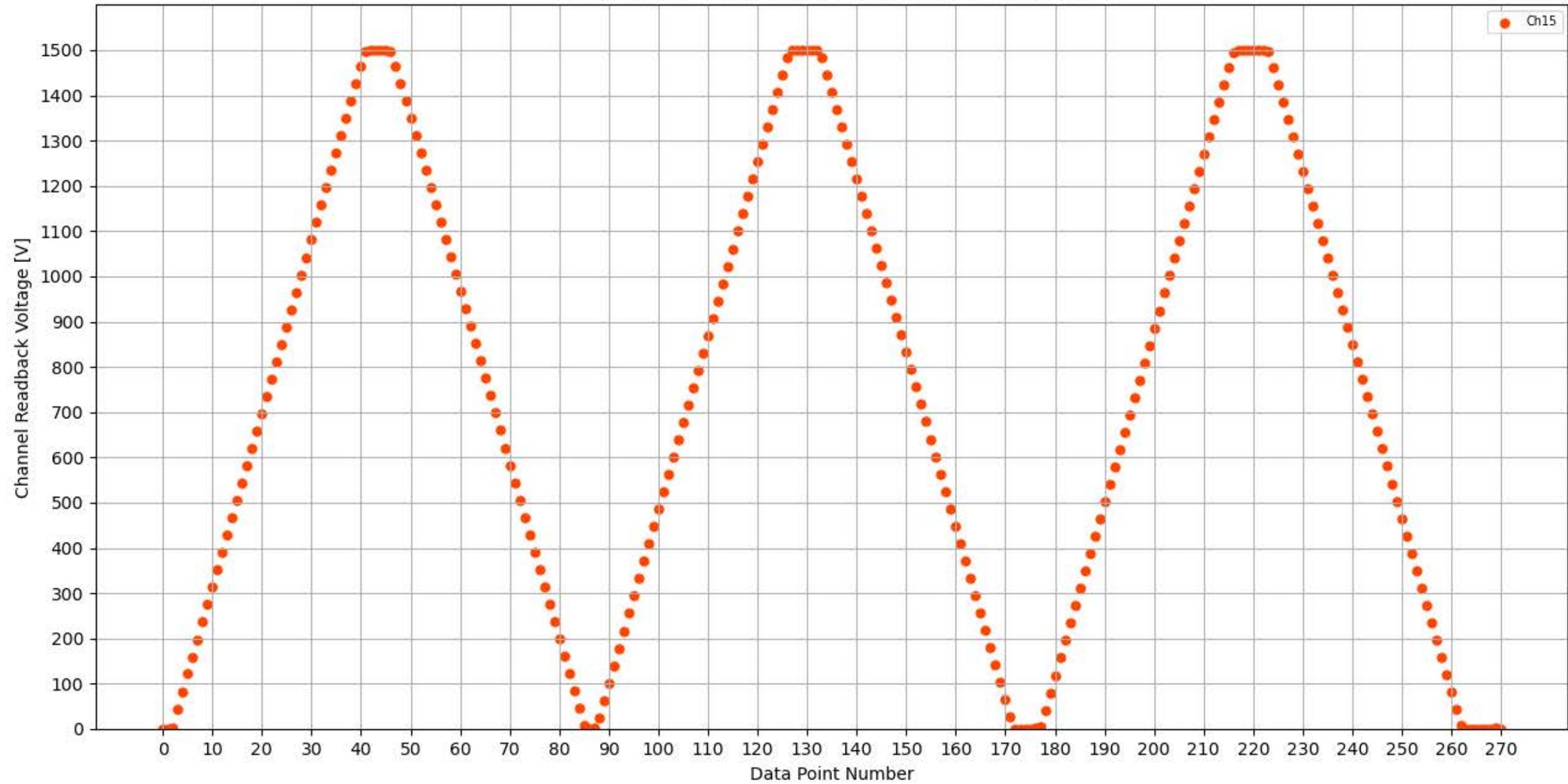
Voltage Ramp Test (Python) Bd #336, Slot #15, Ch #15
