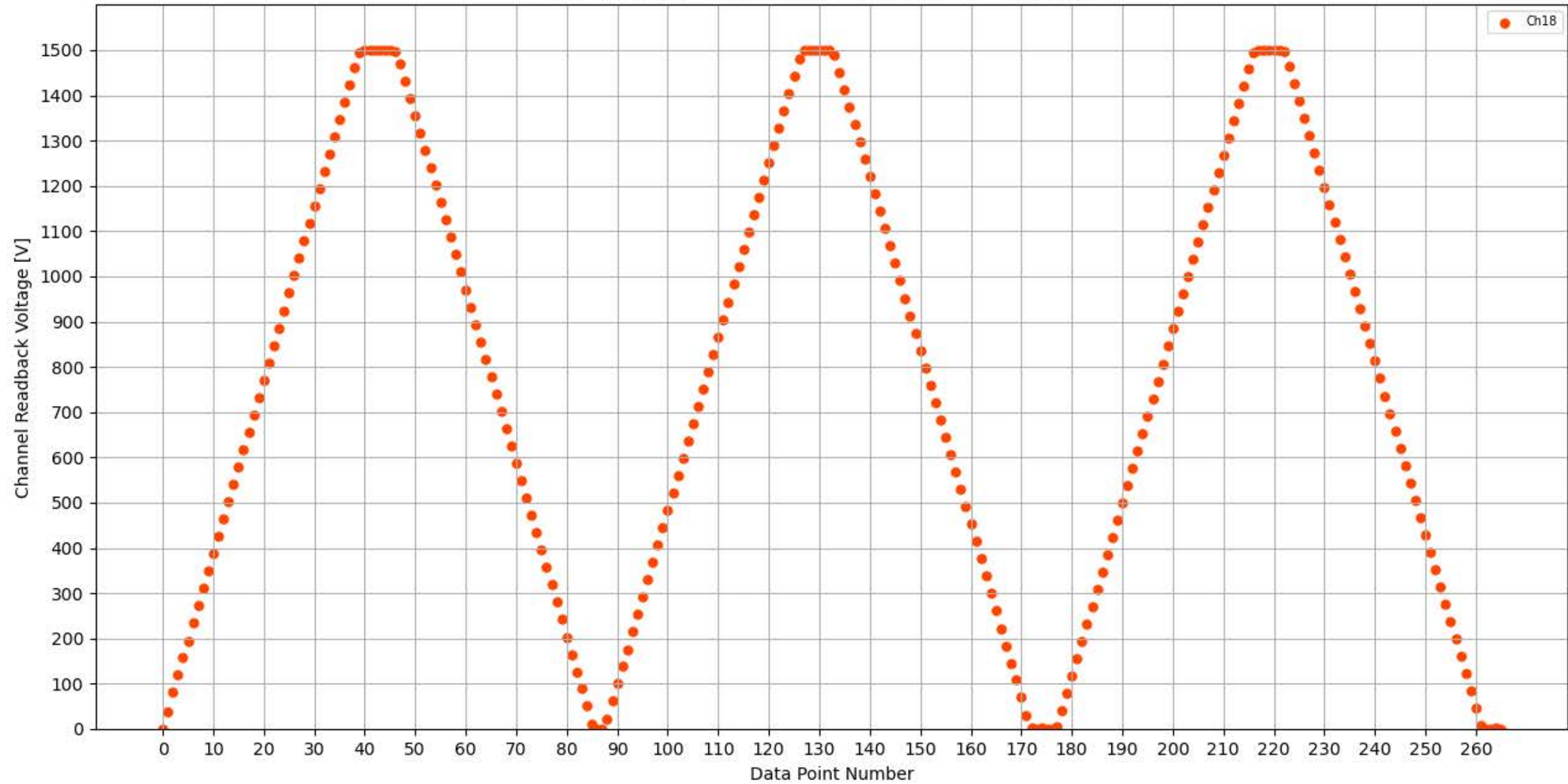
Voltage Ramp Test (Python) Bd #336, Slot #15, Ch #18
