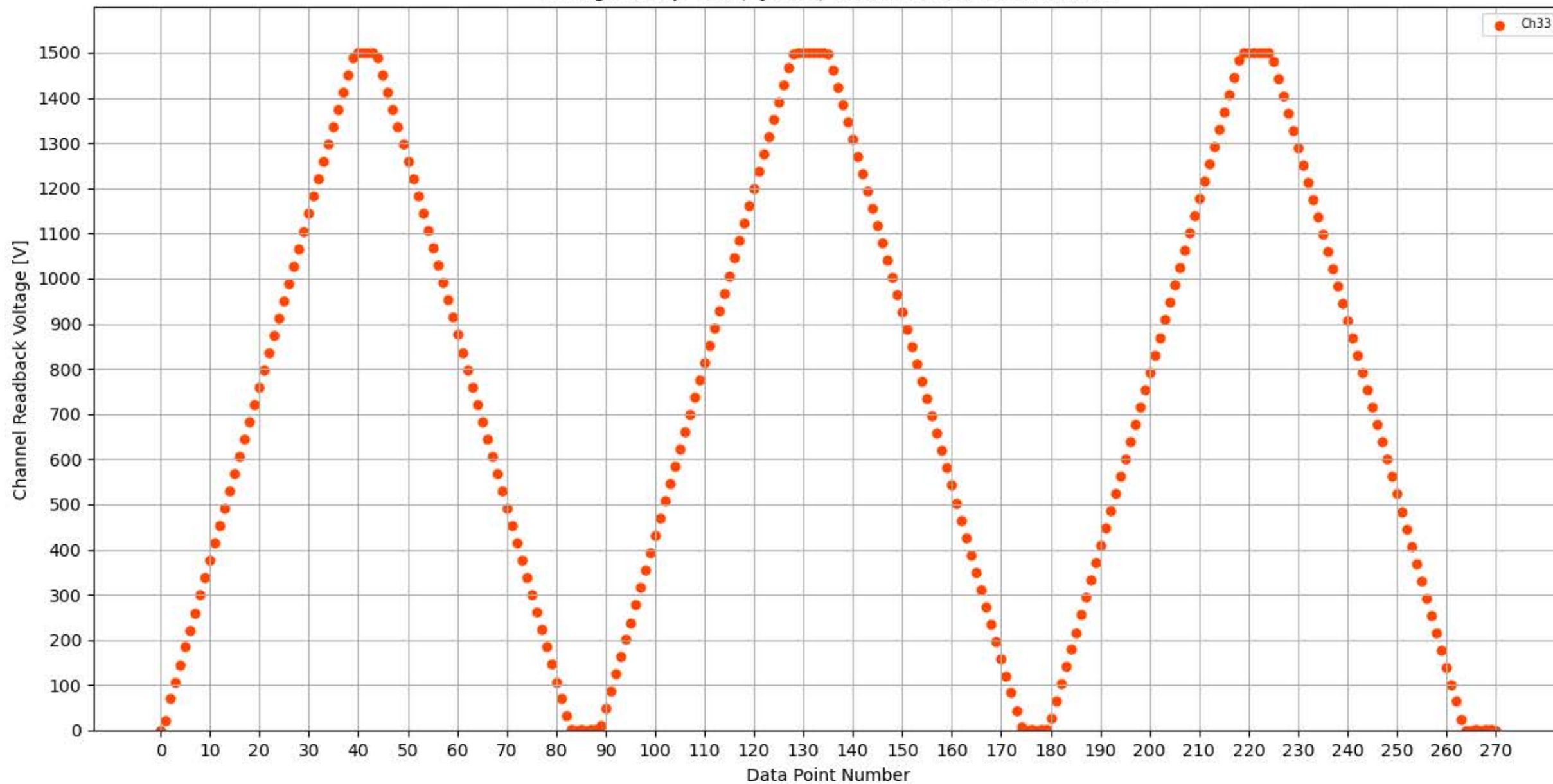
Voltage Ramp Test (Python) Bd #336, Slot #15, Ch #33
