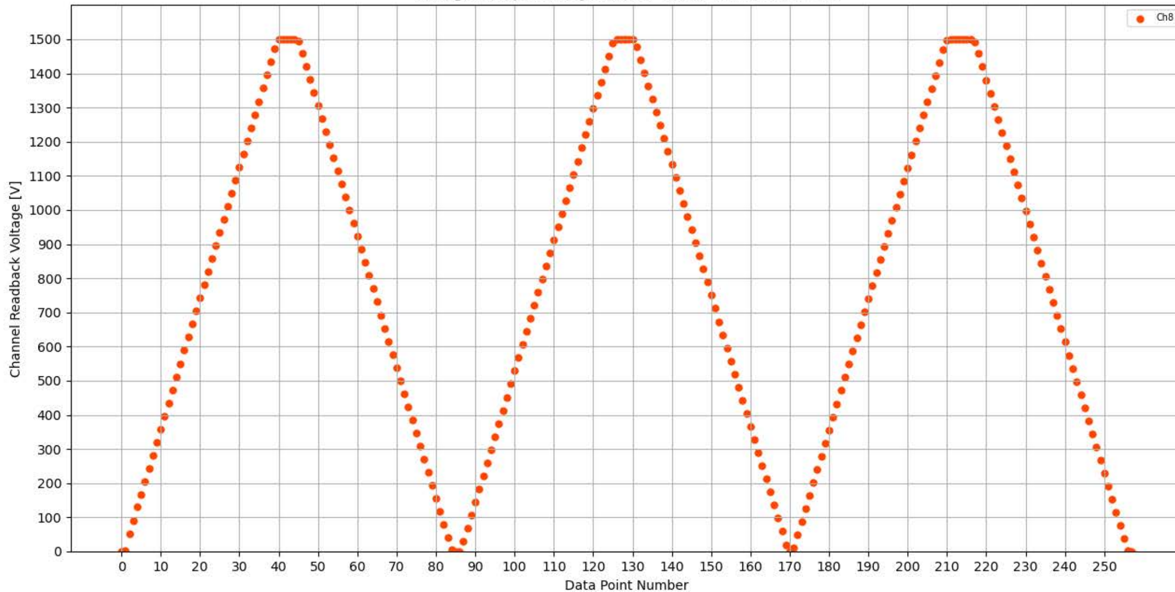
Voltage Ramp Test (Python) Bd #336, Slot #15, Ch #8
