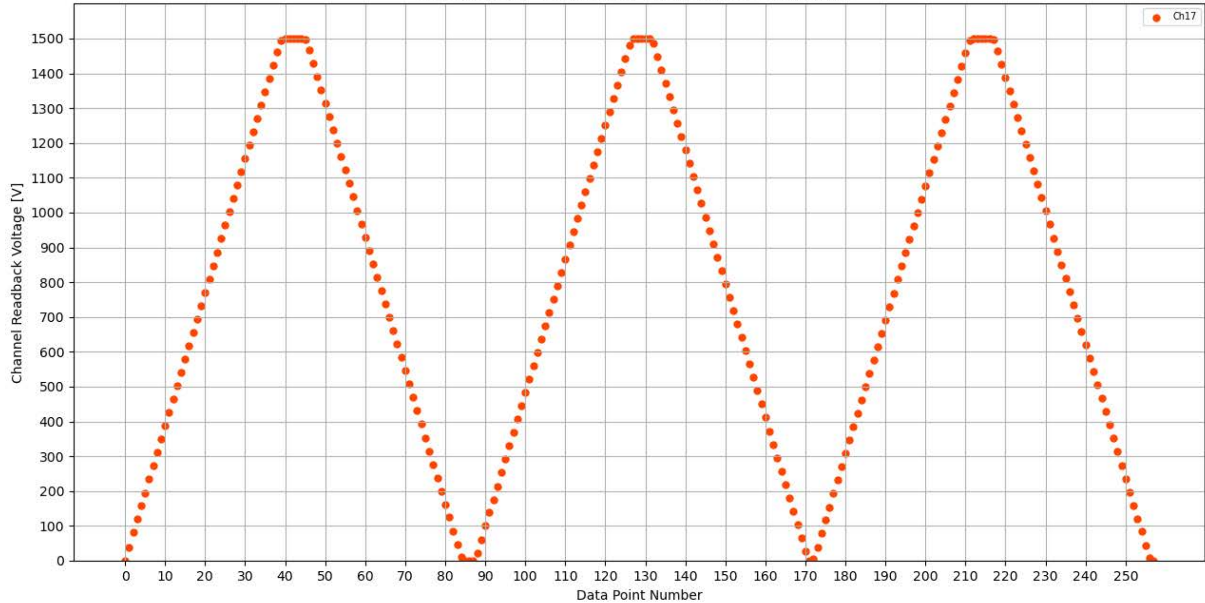
Voltage Ramp Test (Python) Bd #336, Slot #15, Ch #17
