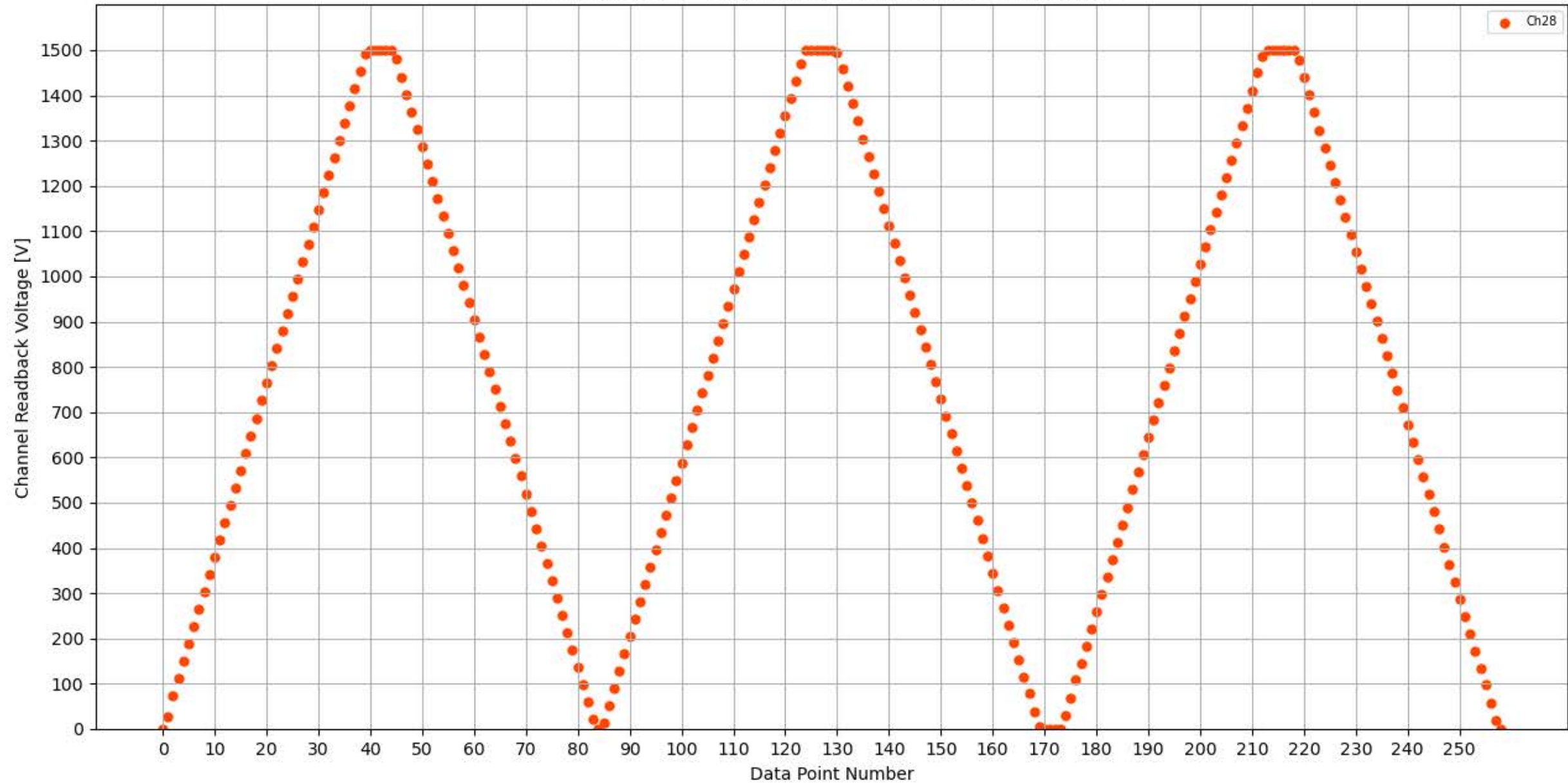
Voltage Ramp Test (Python) Bd #336, Slot #15, Ch #28
